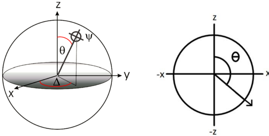
Fig. 10: Bloch sphere. Using equation (4) an arbitrary (normalized) state of the two-dimensional Hilbert space can be parameterized by the two spherical polar coordinates \theta and \Delta . Hereby, \Delta corresponds to a phase shift of the two superposing states \varphi_{\uparrow} and \varphi_{\rightarrow} . On the right hand side, a "Bloch circle" is shown resulting from the assumption of a zero phase shift ( \Delta = 0 ).
