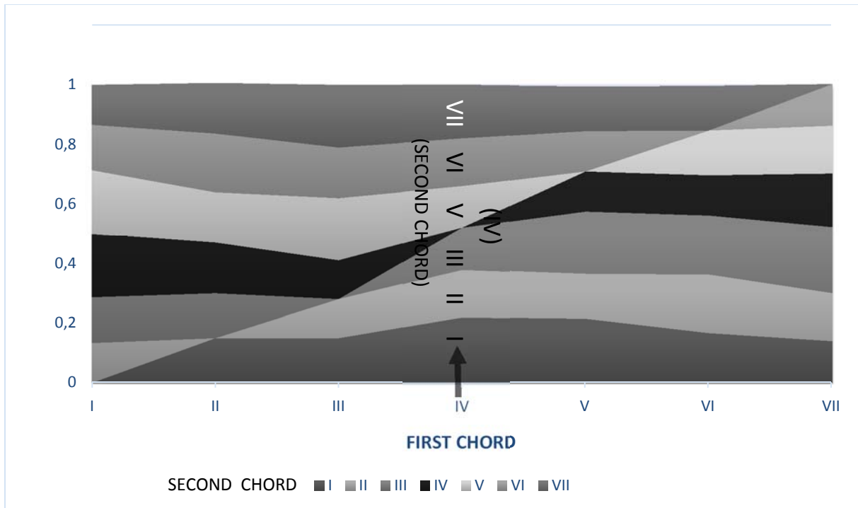
Fig. 6: Stacked chart based on Lerdahl's (1988) model. The calculated conditioned probabilities are inversely related to the distances predicted by the model.
