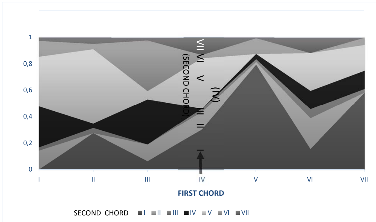
Fig. 5: Stacked chart using corpus data of a sample of baroque music (data from Huron 2006: 251)
