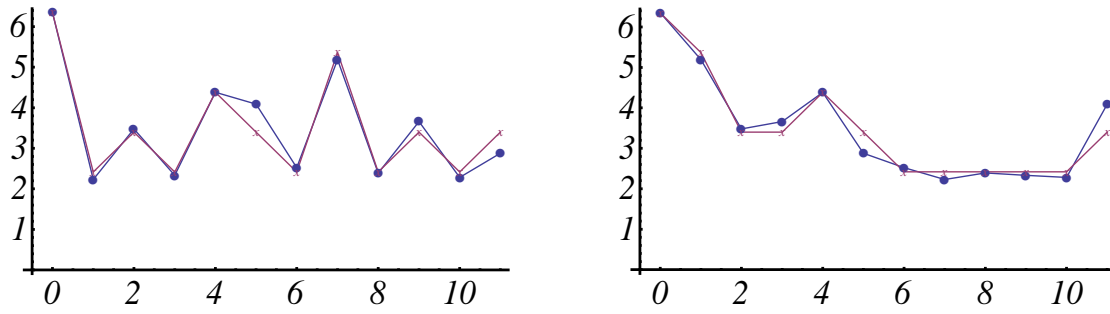
Fig. 1: Distribution marked by \bullet : data of Krumhansl & Kessler (1982) for the key C major; distribution marked by \times : score of constraint violations d fitted to the data of Krumhansl & Kessler (1982) by using the linear approximation 6.5– c . The fit gives the value 6.5 for pitch class 0 (minimal violations) and the value 2.5 for pitch class 1 (maximal violations). On the left hand side, the tones are ordered chromatically; on the right hand side, they are ordered by the ascending circle of fifth.
