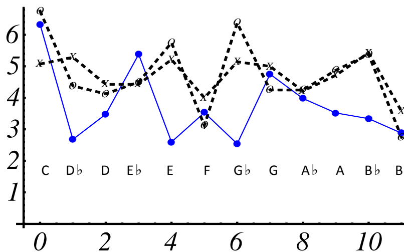
Fig. 8: Full context-driven ICP-profile, where the contexts are (i) the harmonic C-minor scale (dashed profile marked by x) and (ii) the chord G^7 (dashed profile marked by o). The solid curve represents the data of Krumhansl & Kessler (1982) for all 12 pitch classes. The scaling factors are identical with those of Fig. 7
