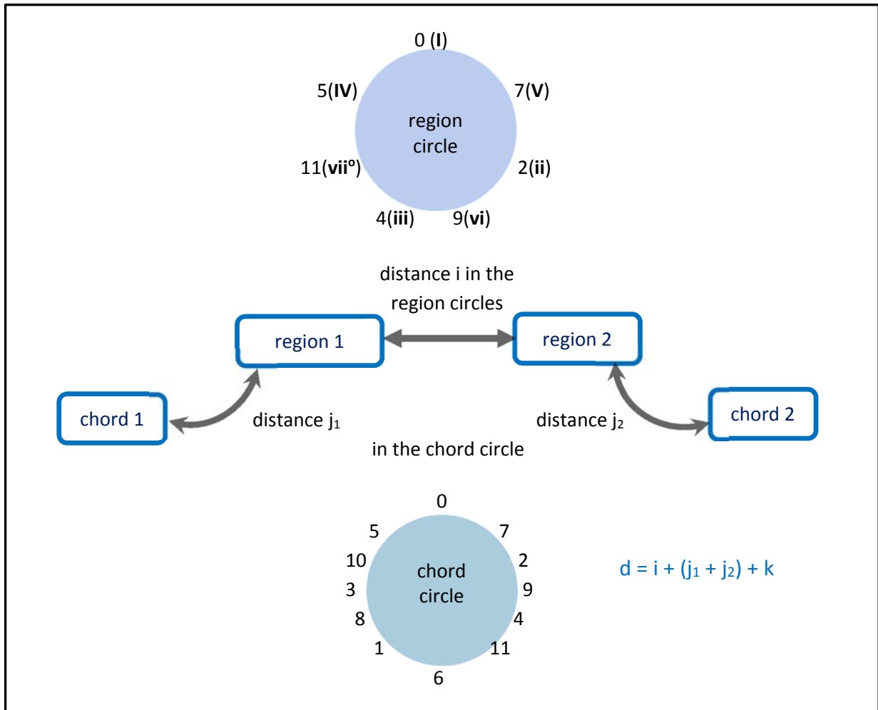
Fig. 4: The chord circle of fifths (bottom) and the region circle of fifths (top) are used to calculate the distance between two chords in Lerdahl's (1988) model of chord proximity.
