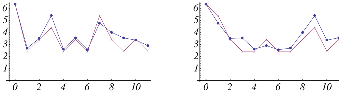
Fig. 2: Related distributions for the key C minor. The harmonic minor scale is chosen for defining the level D violations. On the left hand side, the tones are ordered chromatically; on the right hand side, they are ordered by the ascending circle of fifth.
