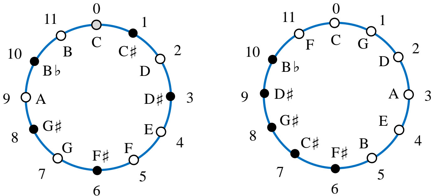
Fig. 11: Visual representation of \mathbb{Z}_{12} . On the left hand side the different elements of the group are generated by the semi-tone generator. The white dots give an ordered subset of \mathbb{Z}_{12} starting with the tone 0. It is the diatonic scale of C-major. On the right hand side, the group elements are generated by a generator that transposes by seven semi-tones (resulting in the circle of fifth). The numbers indicate how often the generator is applied recursively. The tones in the inner circles are the results of application of the corresponding group element to the basic pitch class C.
