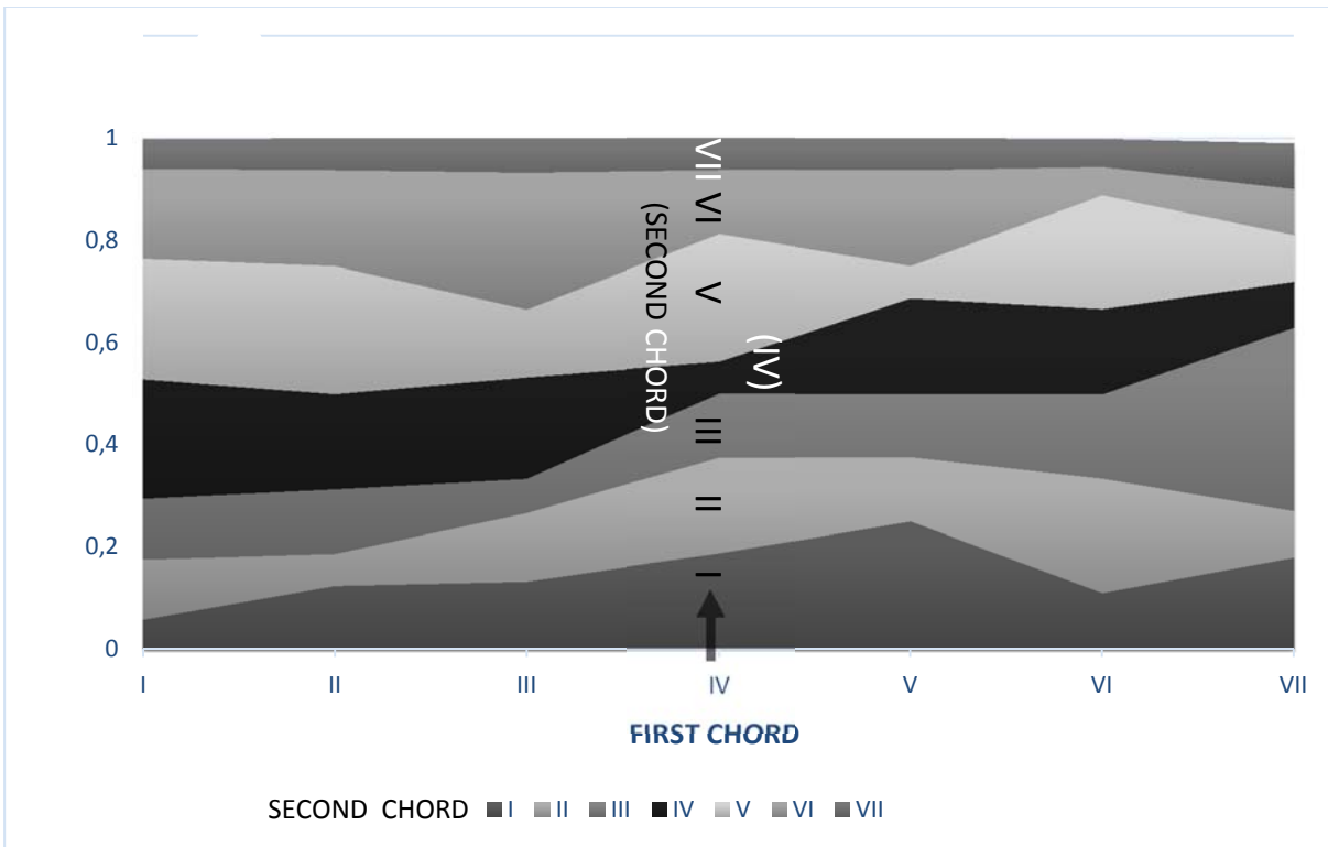
Fig. 9: Stacked chart reflecting Piston's table of chord progression.
