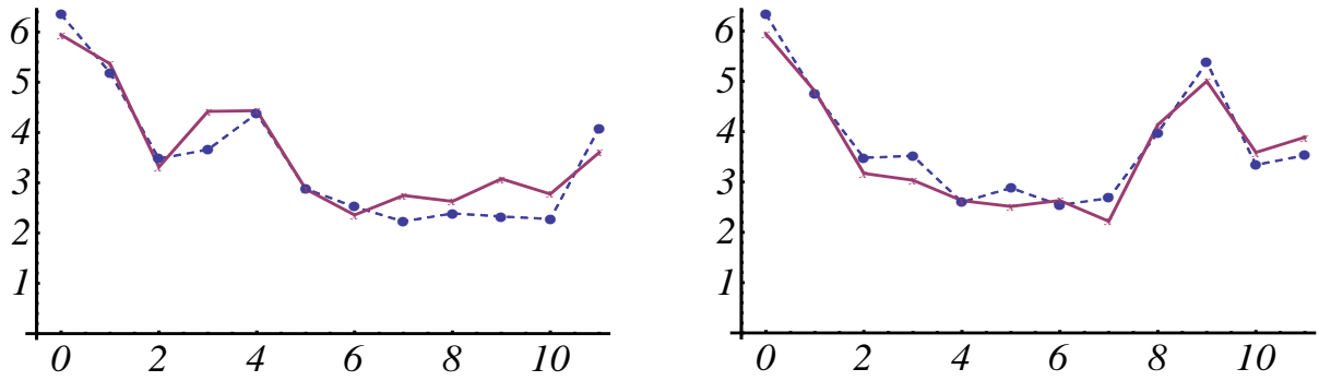
Fig. 14: Comparison of the KK key profiles with the data from the quantum model with fitted phase factors. The dashed curves show the KK key profiles (left: major keys; right: minor keys). The bold curves are the theoretical predictions
