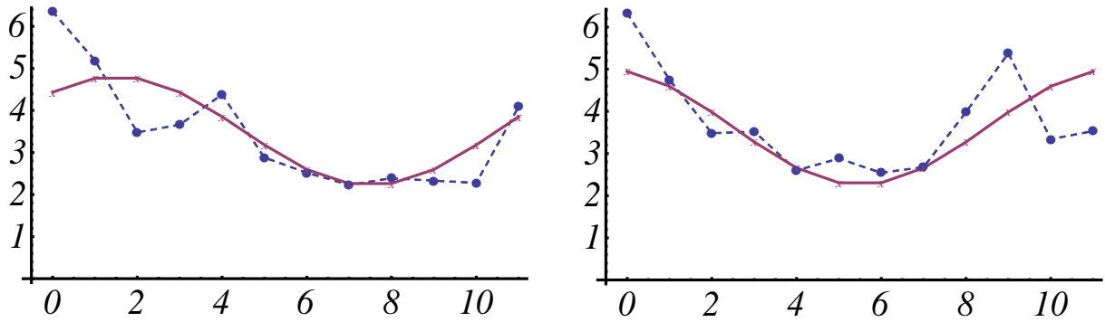
Fig. 13: The dashed curves show the Krumhansl-Kessler profiles (left: major keys; right: minor keys). The bold curves are the theoretical predictions of the quantum model.
