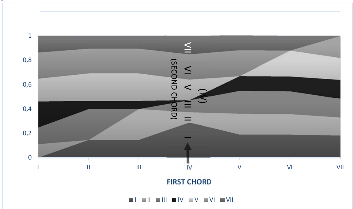
Fig. 15: Stacked chart based on the quantum model with zero phases.
