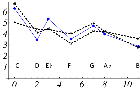
Fig. 7: Context-driven ICP-profile for the harmonic minor scale. The contexts are (i) the harmonic C-minor scale (dashed profile marked by x) and (ii) the chord G^7 (dashed profile marked by o). The distribution marked by • represents the data of Krumhansl & Kessler (1982) for the harmonic minor scale (C-minor). The theoretical curves are scaled for best agreement with the empirical data.
