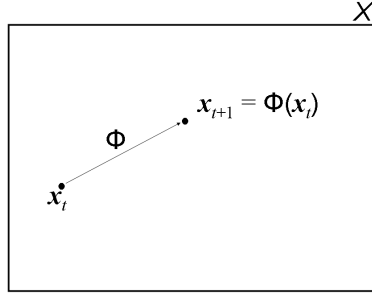
Fig. 3. A discrete-time dynamics of a classical system is given by a map \Phi : X \rightarrow X which assigns to a state \mathbf{x}_t at time t its successor \mathbf{x}_{t+1} = \Phi(\mathbf{x}_t) at time t + 1 .
